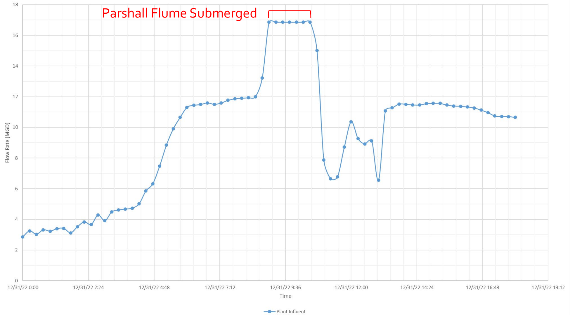
Time Series of Plant Influent Flow Rate on December 31, 2022
